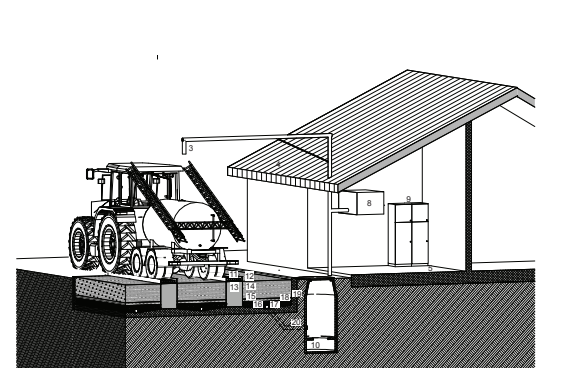
Figure 10: coupe du Biobed.
